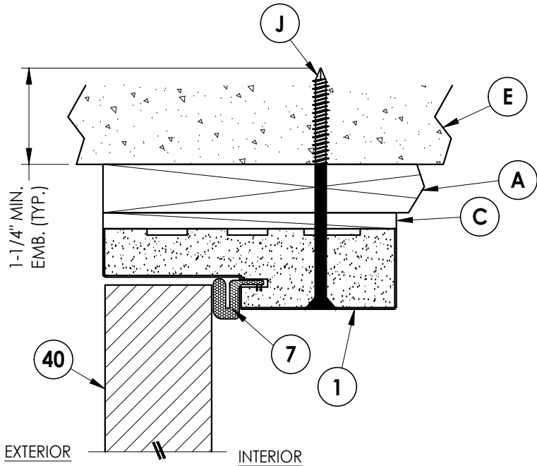
1 6 VERTICAL CROSS SECTION Outswing shown 1X Buck Construction
