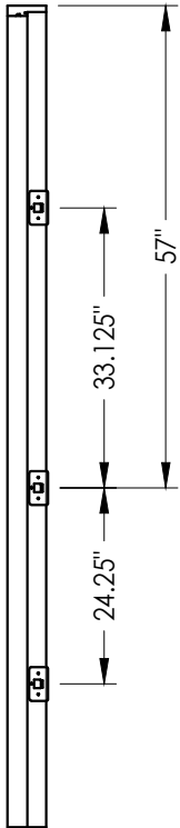
STRIKE JAMB/MULLION MULTI-POINT LOCK
