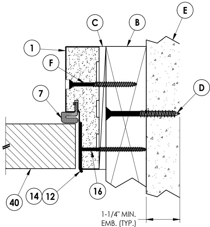
4 5 HORIZONTAL CROSS SECTION Outswing shown 2X Buck Construction
