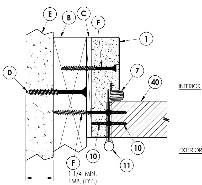
3 5 HORIZONTAL CROSS SECTION Outswing shown 2X Buck Construction
