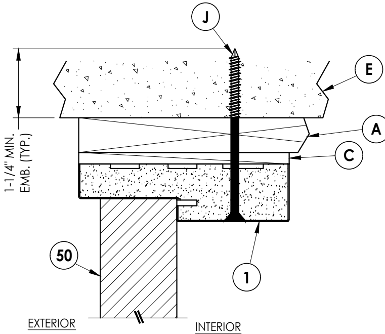
2 6 VERTICAL CROSS SECTION Outswing shown 1X Buck Construction
