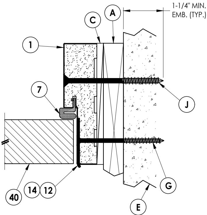
4 6 HORIZONTAL CROSS SECTION Outswing shown 1X Buck Construction
