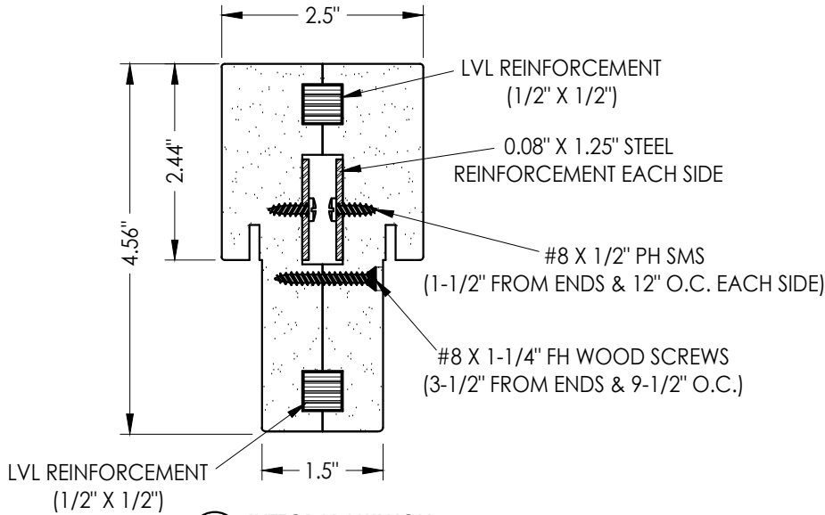
2 INTEGRAL MULLION
