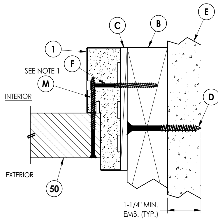
5 5 HORIZONTAL CROSS SECTION Outswing shown 2X Buck Construction
