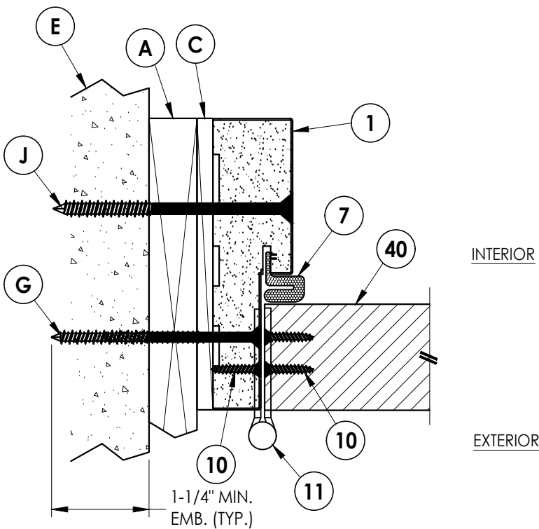
3 6 HORIZONTAL CROSS SECTION Outswing shown 1X Buck Construction
