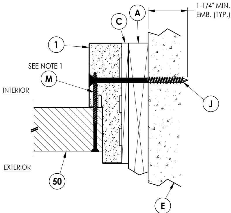
5 6 HORIZONTAL CROSS SECTION Outswing shown 1X Buck Construction
