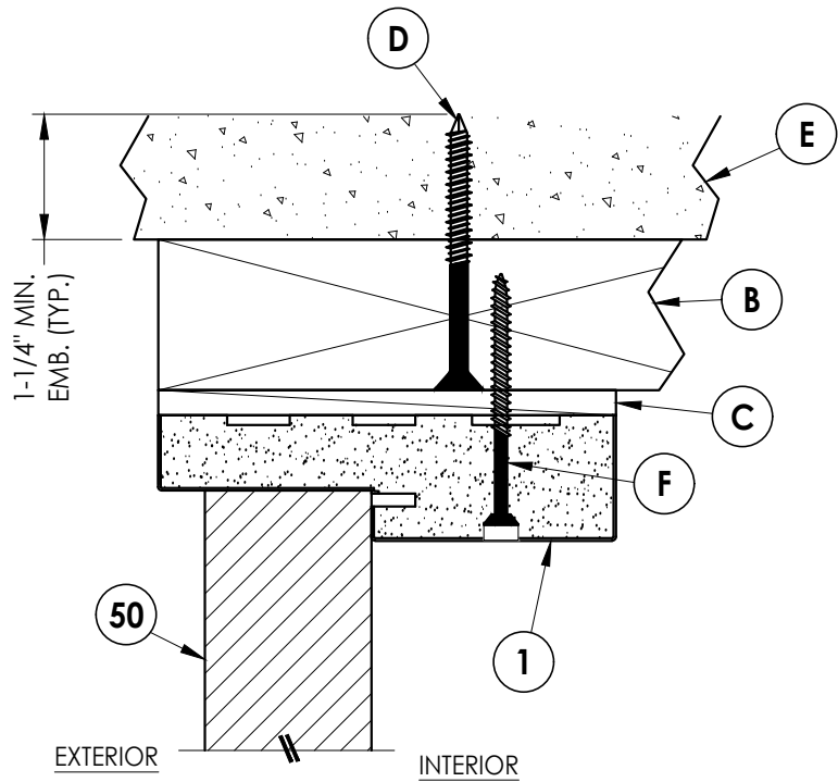
2 5 VERTICAL CROSS SECTION Outswing shown 2X Buck Construction
