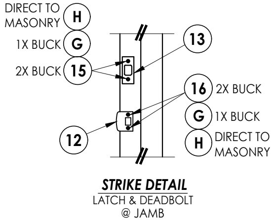
STRIKE JAMB/MULLION LATCH & DEADBOLT
